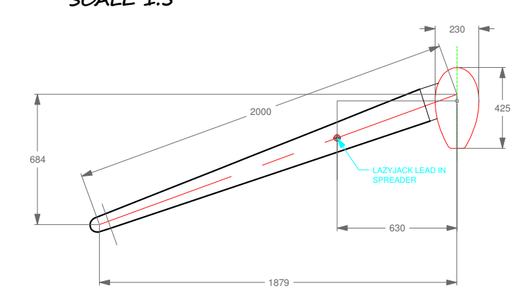
TYPICAL MAST SECTION AND SPREADER SCALE 1:5
